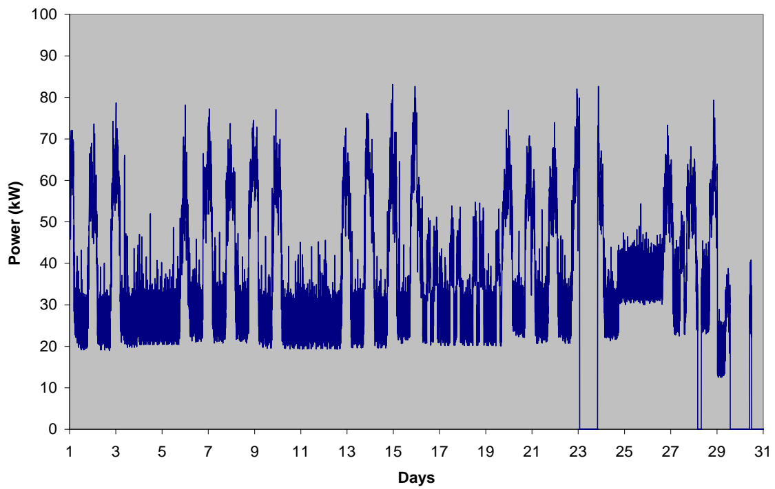
Figure 14. Month 2 facility power.
