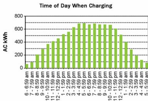
Figure 15: Time of day when charging versus charging energy.
