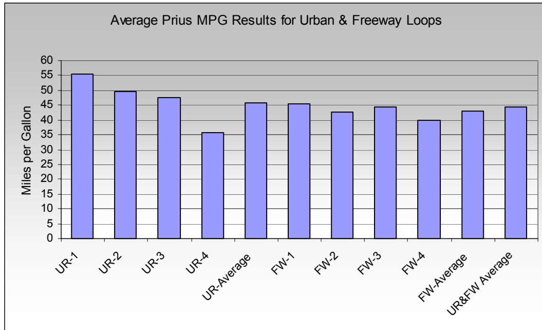
Figure 1. Average miles per gallon (mpg) for each operating scenario used for the Urban and Freeway Pomona Loops.
