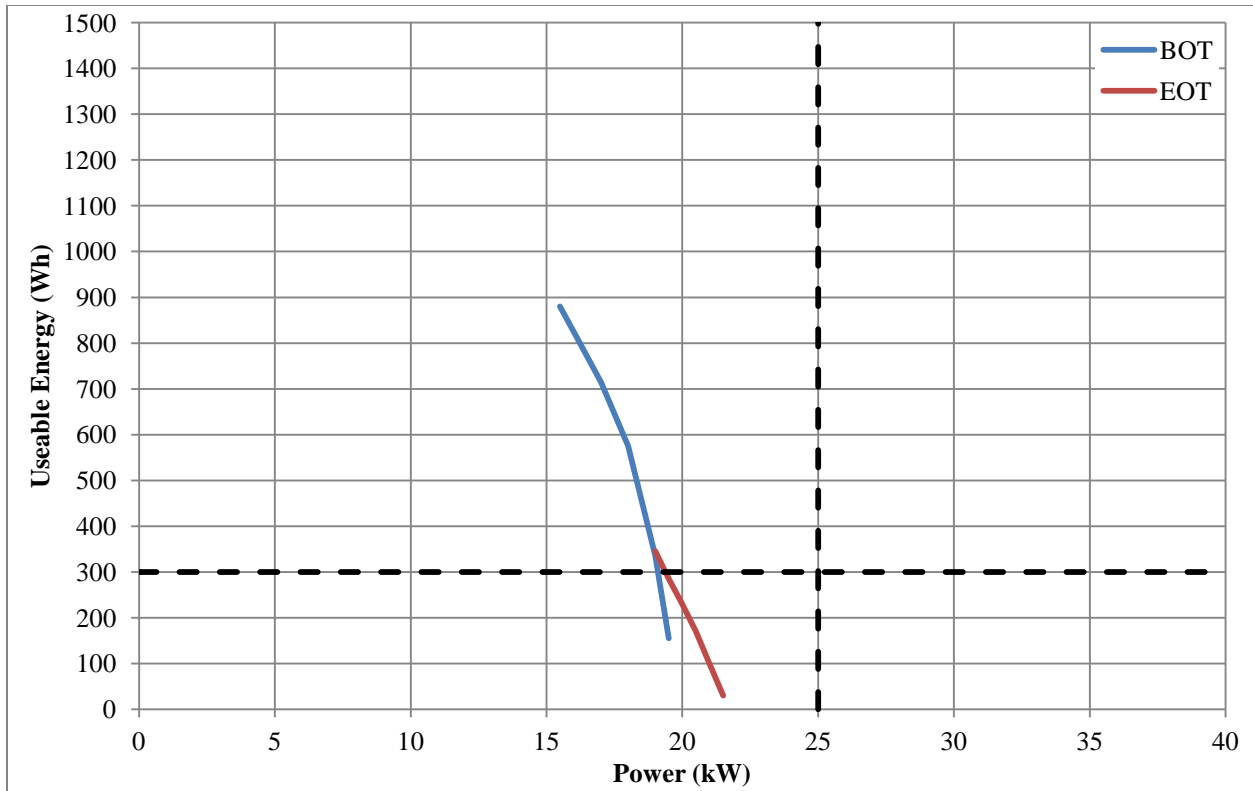
Figure 7. Useable energy versus power.
