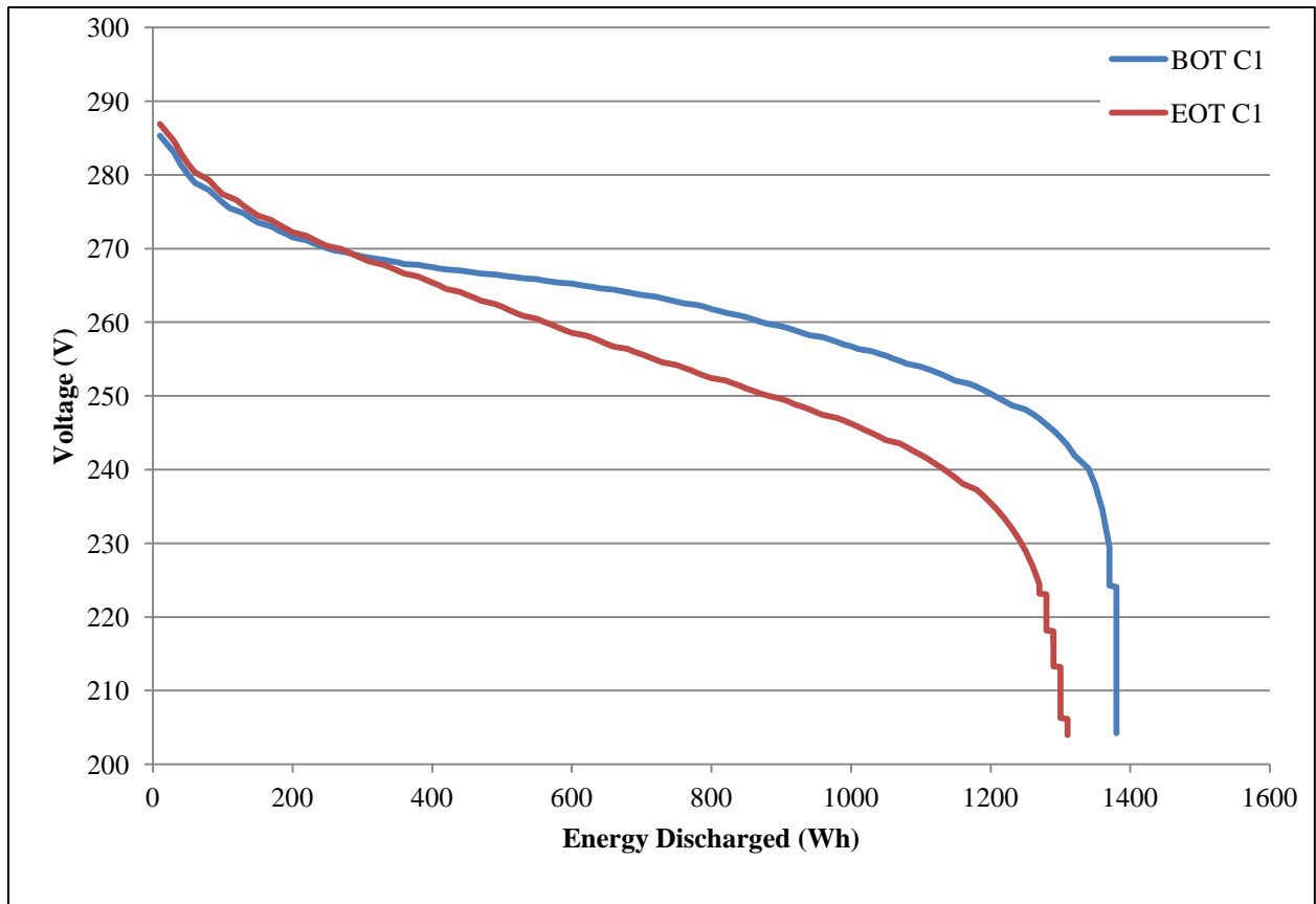
Figure 1. Voltage versus energy discharged during the static capacity test.
