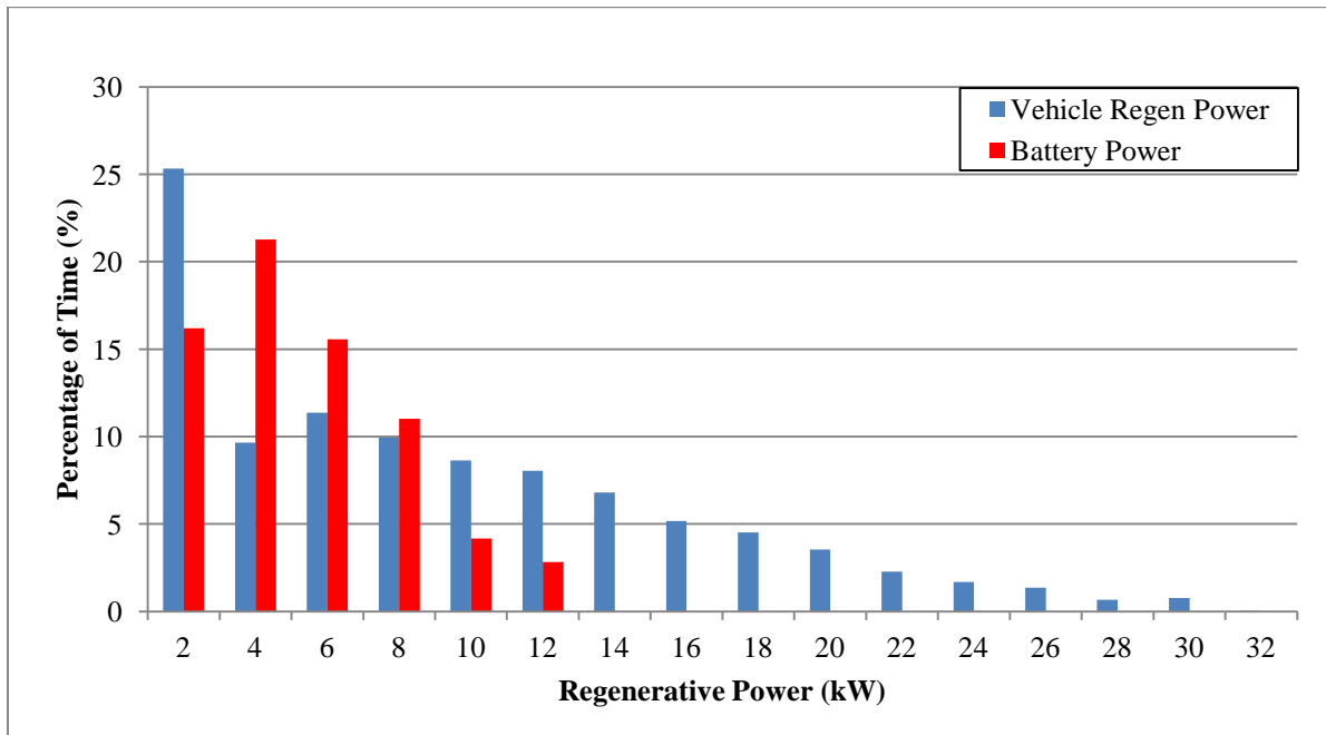
Figure 12. Percentage of time at regenerative power level.
