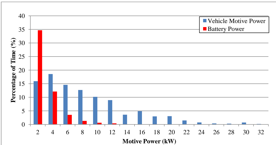
Figure 11. Percentage of time at motive power level.
