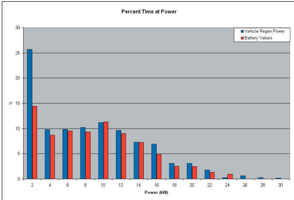
Figure 12. Percent time at regenerative power level.
