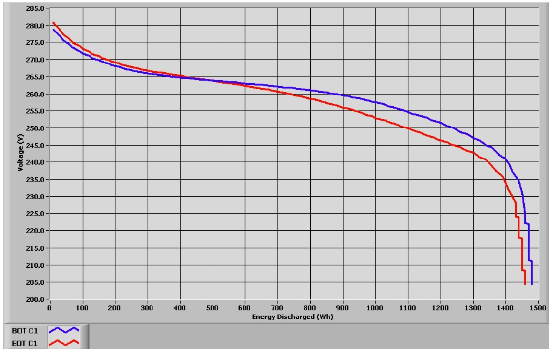
Figure 1. Voltage versus energy discharged.
