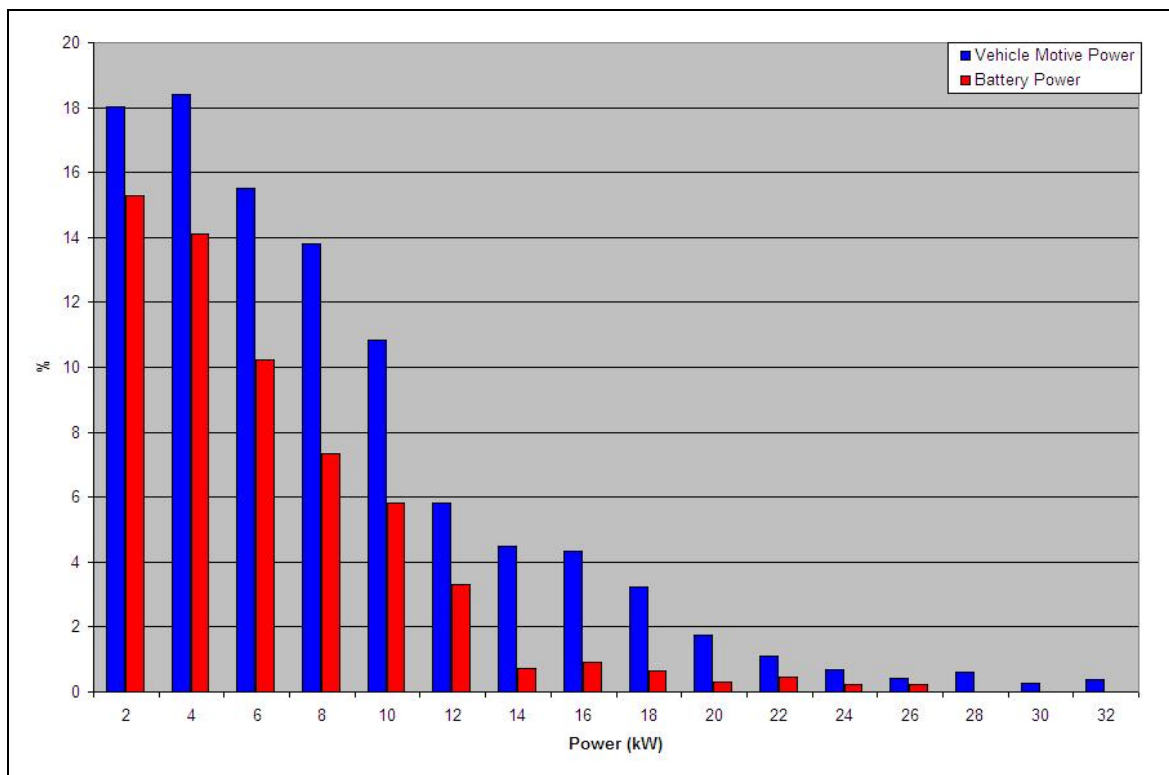
Figure 11. Percent time at motive power level.
