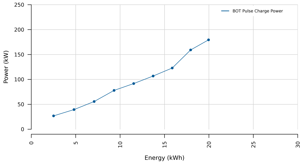
Figure 4. Charge power capability versus energy discharged
