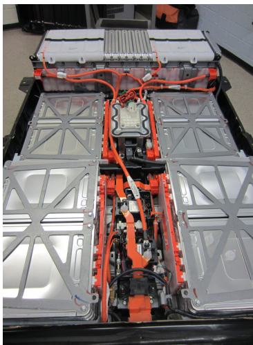
2013 Nissan Leaf battery pack top view when removed from the vehicle
