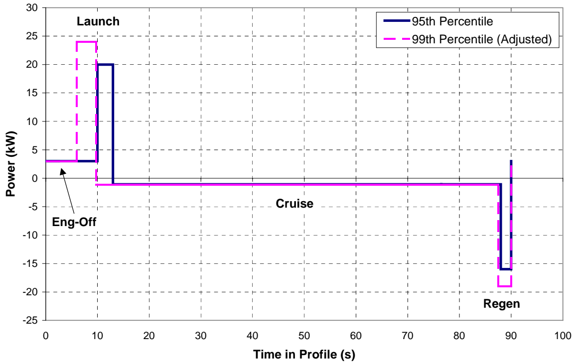
Figure 4. FreedomCAR 95 th and 99 th Percentile cycle-life profiles.
