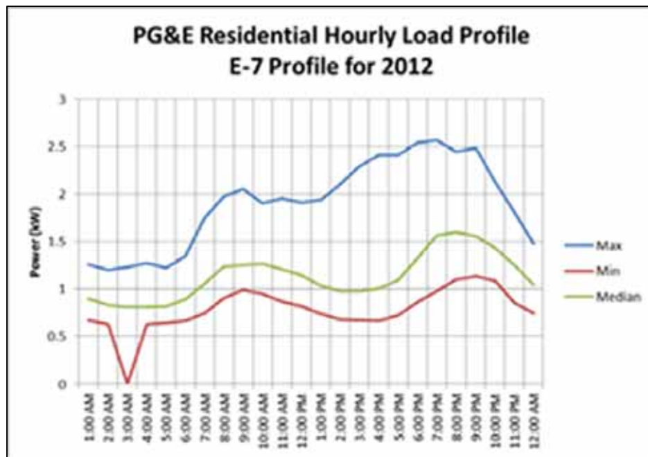
Figure 11-72. PG&E hourly residential load profile.
