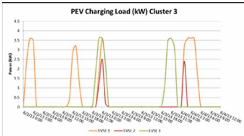
Figure 11-81. PEV Charging Profile for Cluster Site 3.
