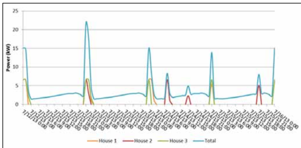
Figure 11-69. Hourly load profile for Cluster Site 3 with 6.6-kW charging.
