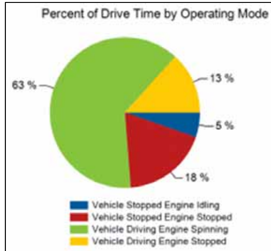
Figure 8-33. Percent of drive time when the Ram's gasoline engine was either stopped, spinning, or idling.
